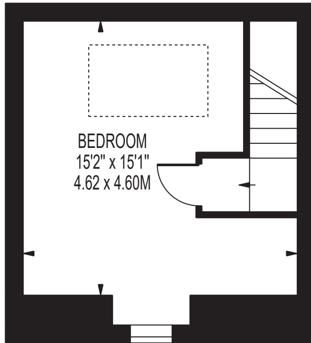
TOP FLOOR
